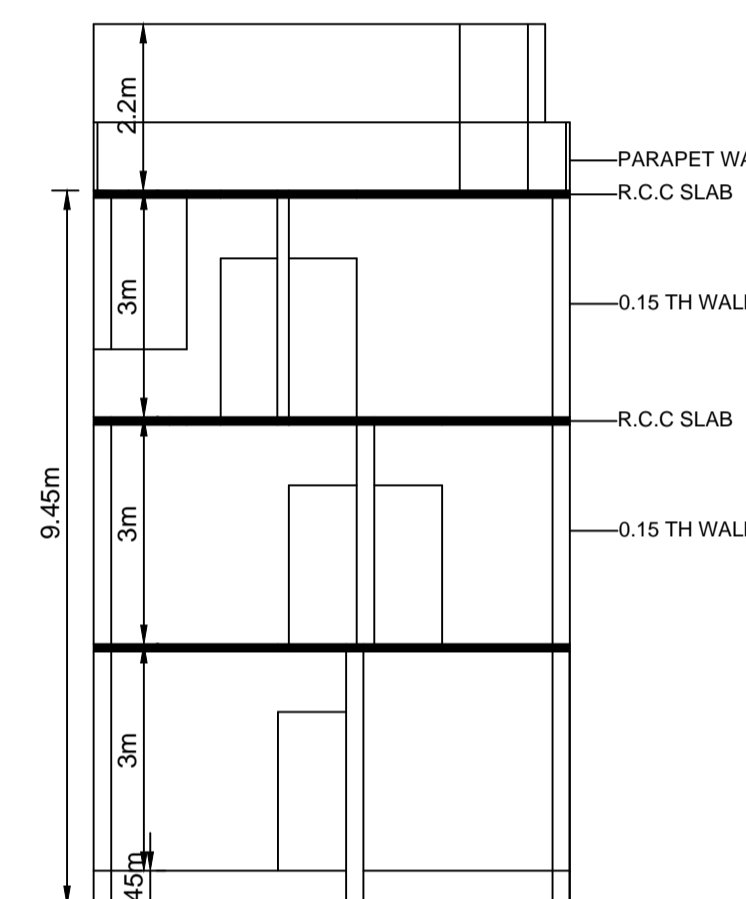
SECTION @ X-X
