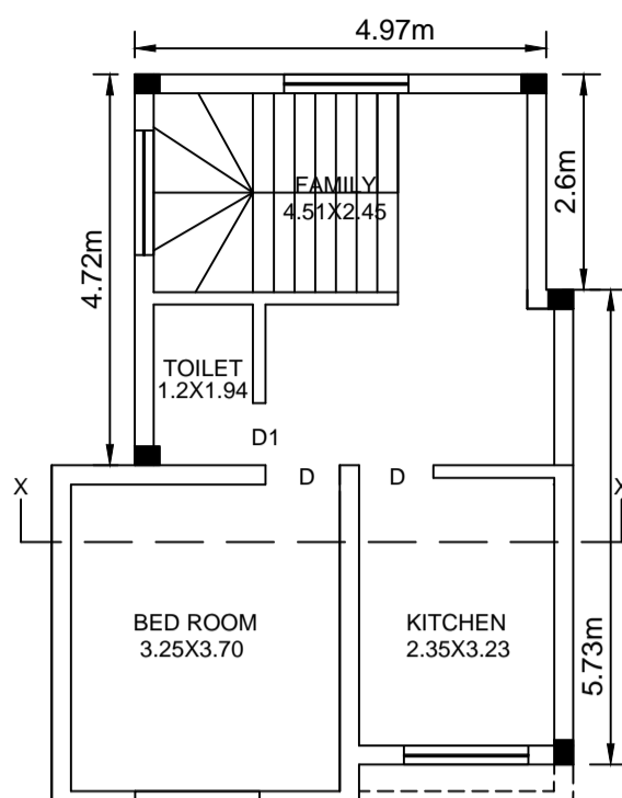
PROPOSED ADDITION & ALTERATION TO EXISTING FIRST FLOOR PLAN
